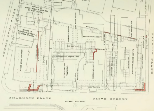
PLAN OF THE OLD FORT WITH THE EXISTING BUILDINGS, 1903.
